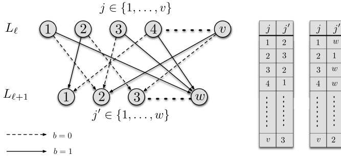
Fig. 1. An arbitrary level in a fragment of branching program (on the left) and the corresponding tables (on the right). The choice of a table depends on U 's input b .
