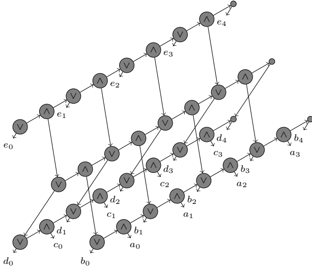
Fig. 1. Circuit resulting from unrolling the LTL formula ((a \cup b) \cup (c \cup d)) \cup e over a path \rho of length 5. We denote the value of an atomic proposition p at a path position i = 0, \dots, 4 by p_i . The graph of the circuit has no planar embedding.
