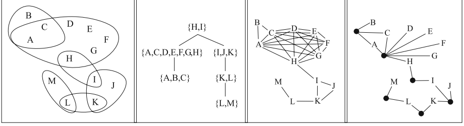
Fig. 2. A hypergraph \mathcal{H}_1 , a join tree JT(\mathcal{H}_1) , the primal graph G(\mathcal{H}_1) , and the incidence graph inc(\mathcal{H}_1)
