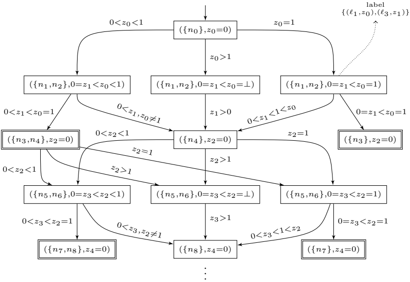
Fig. 3. The DAG induced by the infinite timed tree \text{SymbDet}(R(\mathcal{A}^\infty))
